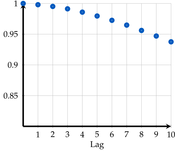
Figure 5: Autocorrelation function of the equilibrium bond sequence
