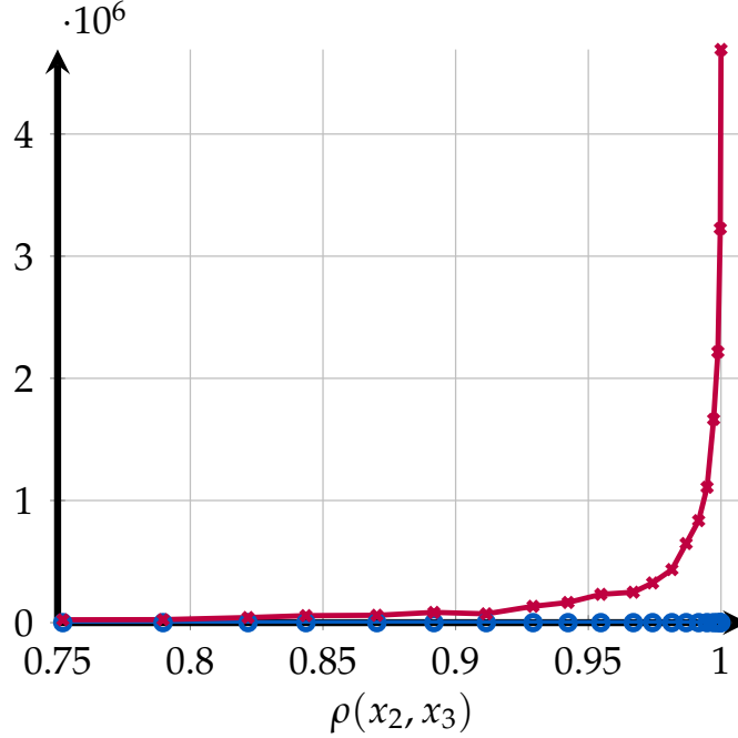
Figure 4: Mean squared prediction error with a neural network and a polynomial
