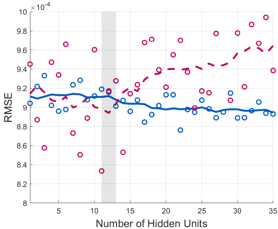
Figure 3: Root Mean Squared Error (RMSE) in function of the number of neurons in the hidden layer Notes: The figure shows the relation between the number of hidden units and neural network performance in the neoclassical growth model. Solid blue line - network performance on the training set. Dashed purple line - network performance on the validation set. Circles show network performance for a specific number of units. Lines represent the moving averages.
