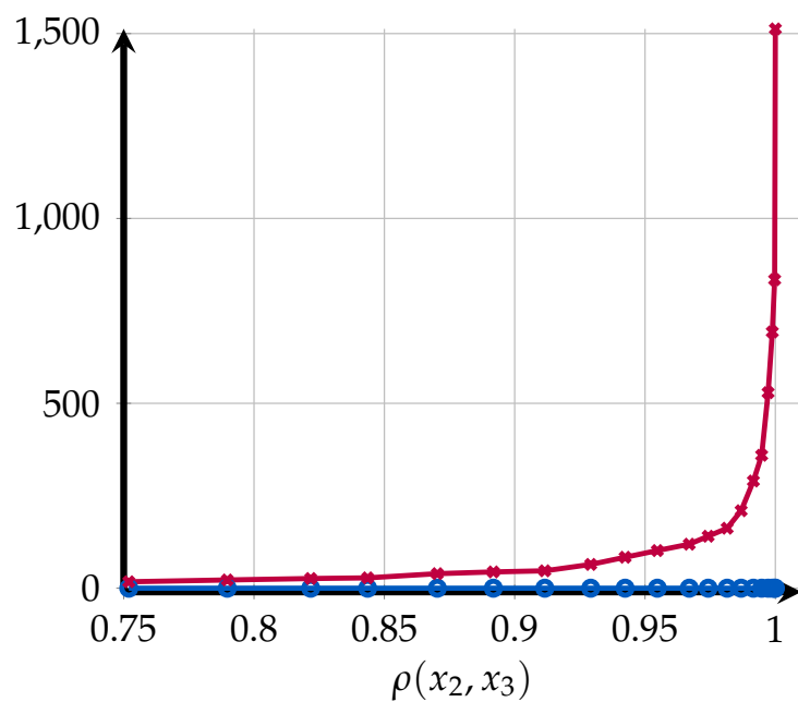
Figure 9: Variance term of the mean squared prediction error with a neural network and a polynomial Notes: The figure shows the variance component of the mean squared prediction error 1/n \sum_{t=1}^n [y_t - \mathbb{E}(\hat{y}_t)]^2 in function of the correlation between x_2 and x_3 . Blue line with circles - NN, purple line with crosses - polynomial regression.
