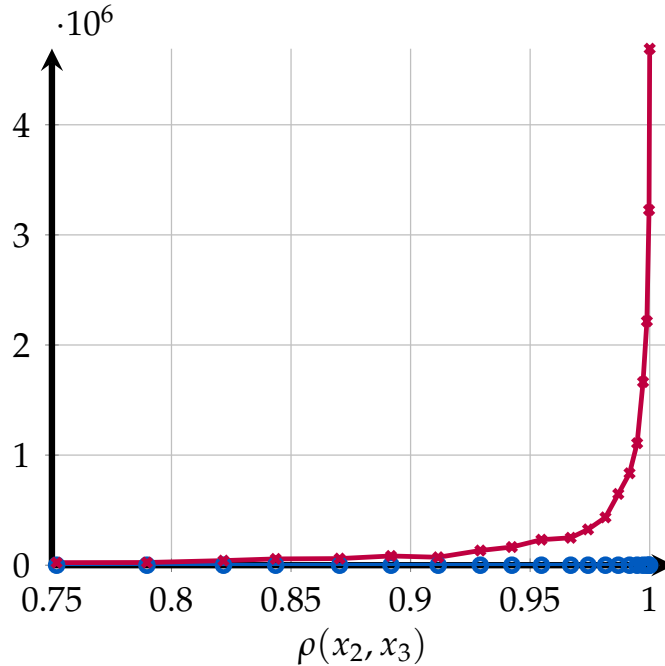
Figure 8: Bias squared of the mean squared prediction error with a neural network and a polynomial Notes: The figure shows the bias squared of the mean squared prediction error 1/n \sum_{t=1}^n [y_t - \mathbb{E}(\hat{y}_t)]^2 in function of the correlation between x_2 and x_3 . Blue line with circles - NN, purple line with crosses - polynomial regression.
