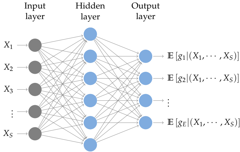
Figure 1: Artificial Neural Network Structure
