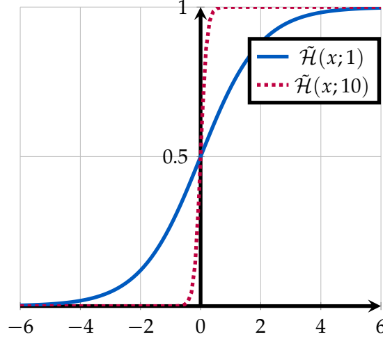
Figure 2: Sigmoid Function
